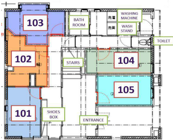
1F
